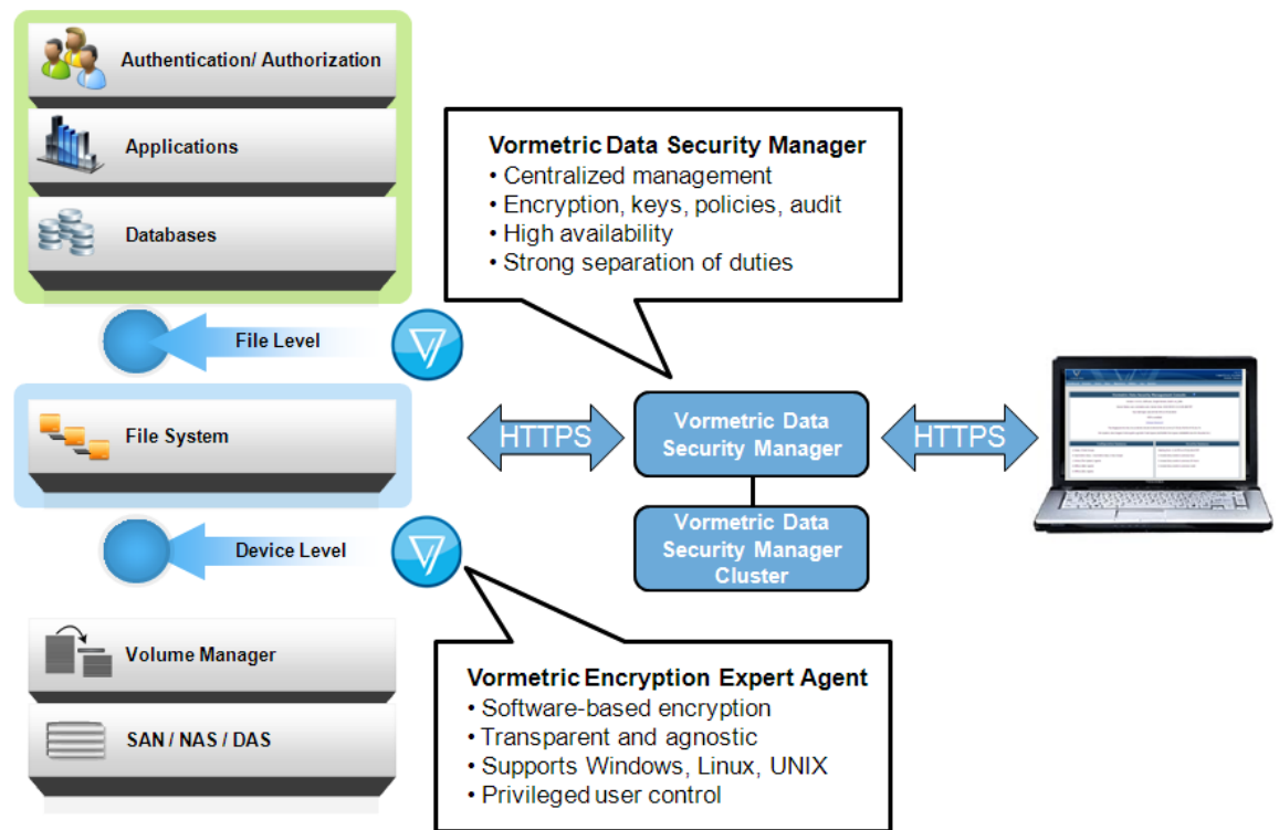
Figure 3: Vormetric Encryption Expert Agents reside between database, application or user layer and file system or volume manager in order to transparently encrypt/decrypt data.
